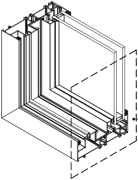
DETAY-9 DETAIL-9
