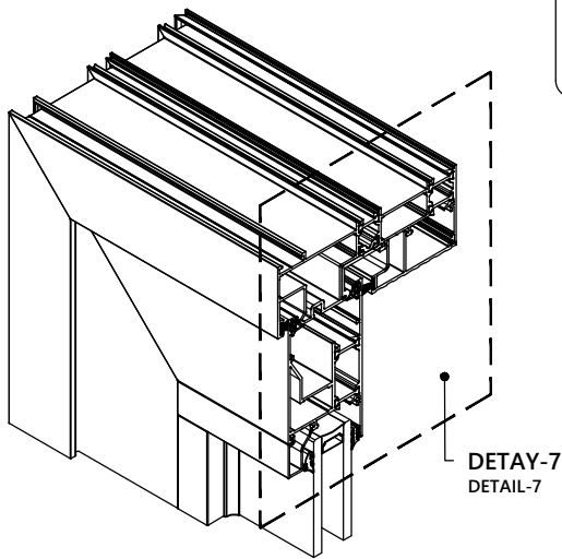
DETAY - 7 DETAIL - 7
