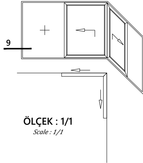
DETAY - 9 DETAIL - 9
