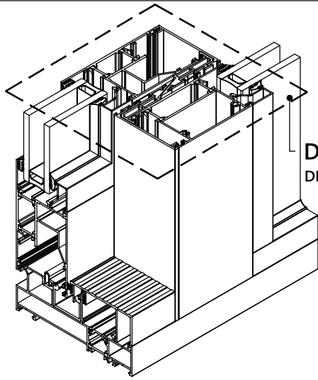
DETAY - 2 DETAIL - 2
