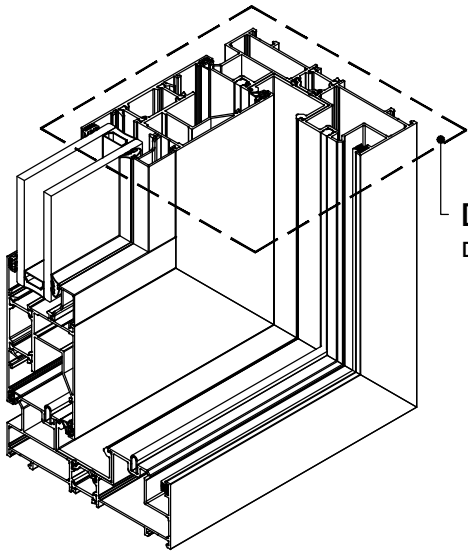
DETAY - 3 DETAIL - 3
