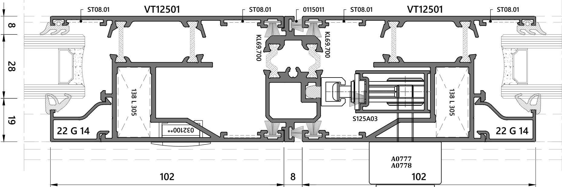
DETAY - 5 DETAIL - 5
