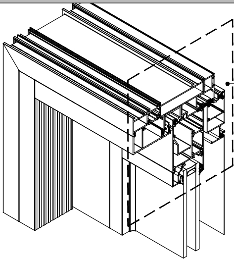
DETAY-12 DETAIL-12
