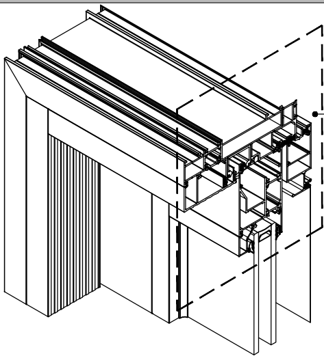
DETAY - 12 DETAIL - 12
