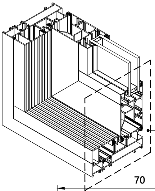
DETAY - 5 DETAIL - 5
