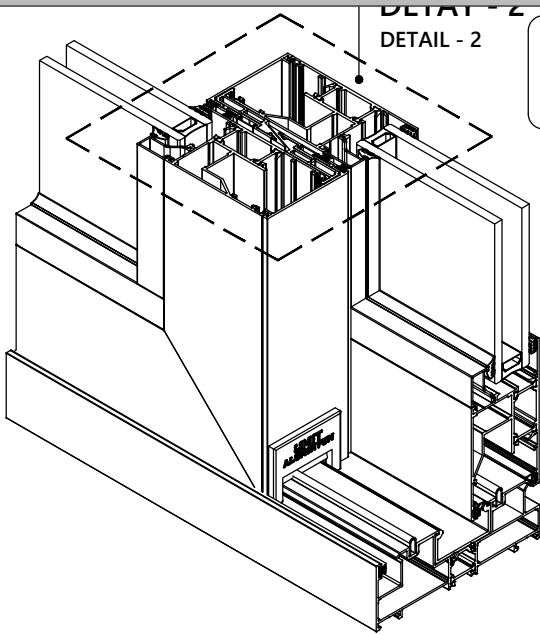
DETAIL - 2 DETAIL - 2
