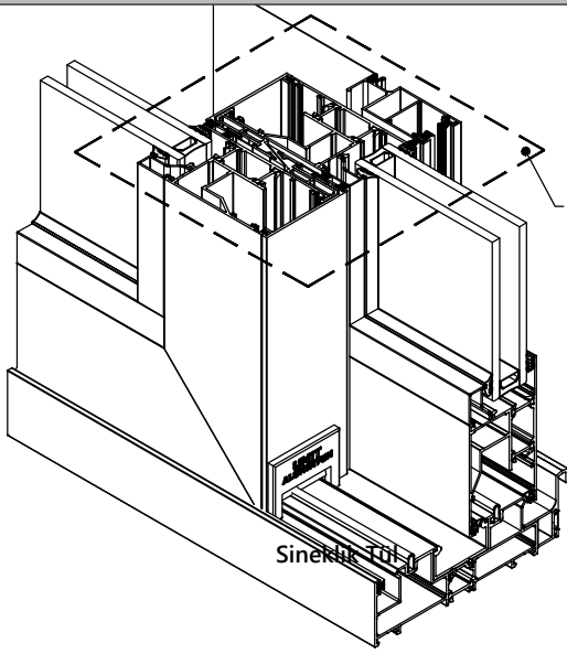
DETAY - 13 DETAIL - 13
