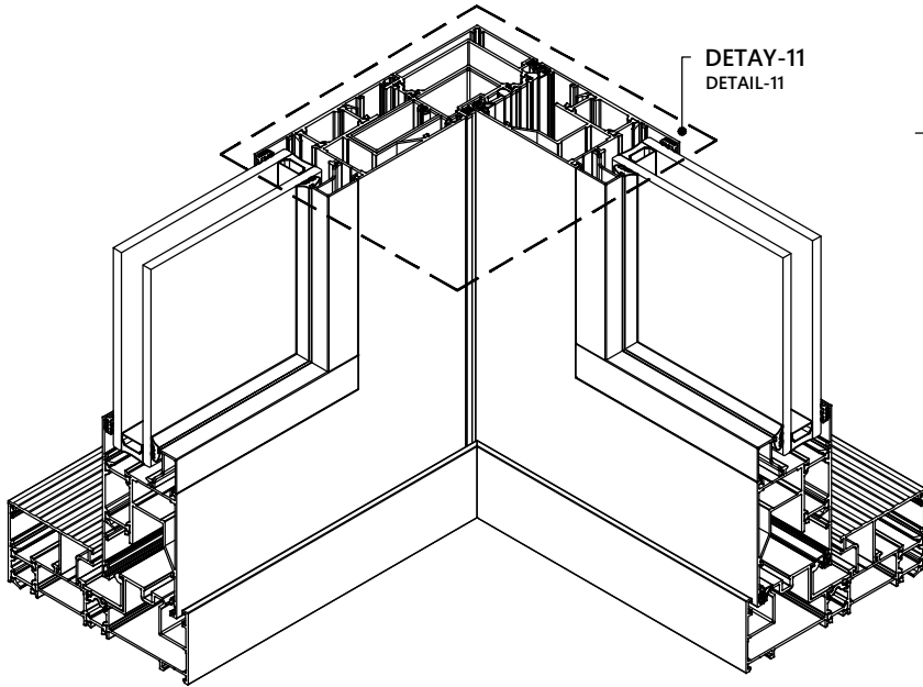
DETAY - 11 DETAIL - 11
