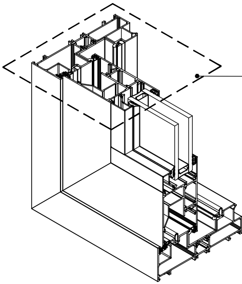
DETAY - 1 DETAIL - 1
