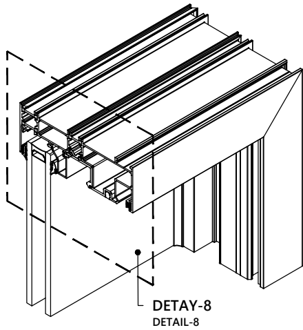
DETAY - 8 DETAIL - 8
