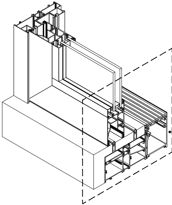
DETAY-11a DETAIL-11a
