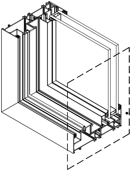
DETAY-9 DETAIL-9
